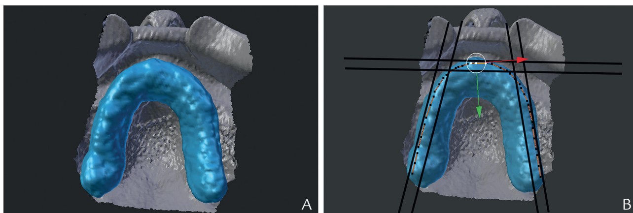
Figure 3. Occlusal view of digital maxilla imported into CAD software. A, Intaglio surface delimitation of maxillary digital baseplate and determination of homogeneous thickness of 2 mm for maxillary digital baseplate. B, Delimitation of rim above digital baseplate. CAD, computer-aided design.
