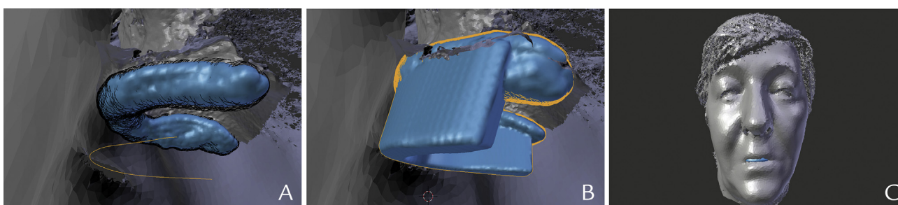
Figure 4. A, Occlusal curve delimitation beyond upper lip. B, Tentative design of maxillary baseplate and rim. C, Frontal view of maxillary baseplate and rim and superimposed with the facial scan.
